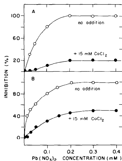
Fig. 1. Inhibition of oxygen evolution ( \text{H}_2\text{O} \rightarrow \text{DCBQ} ) by \text{Pb}(\text{NO}_3)_2 in the absence ( \circ ) and in the presence ( \bullet ) of \text{CaCl}_2 (15 mM). (A) Intact PS II. (B) NaCl-washed PS II. Absolute values for oxygen evolution activity: (A) no addition 366 and +15 mM \text{CaCl}_2 402 \mu\text{mol O}_2/\text{mg Chl/h} ; (B) no addition 107 and +15 mM \text{CaCl}_2 350 \mu\text{mol O}_2/\text{mg Chl/h} .
