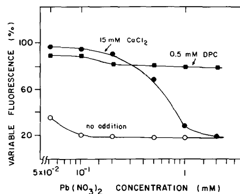
Fig. 5. Quenching of variable fluorescence by \text{Pb}(\text{NO}_3)_2 in intact PS II membranes. No addition (○); \text{CaCl}_2 (15 mM) (●); DPC (0.5 mM) (■).
