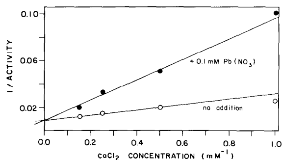
Fig. 3. Double reciprocal plot of the competitive interaction between \text{Pb}(\text{NO}_3)_2 and \text{CaCl}_2 in NaCl-washed PS II membranes. No addition (○) and presence of \text{Pb}(\text{NO}_3)_2 (0.1 mM) (●).
